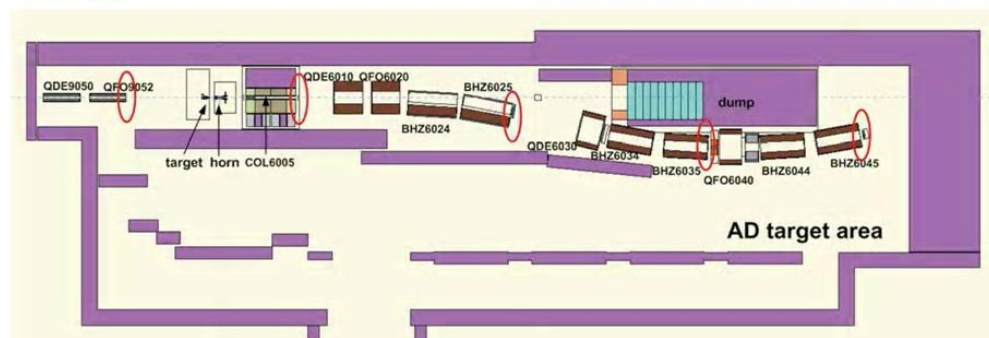
Fig. 2: The AD-target area FLUKA model. The existing BCT positions (downstream the QFO9052 magnet and the COL6005 collimator) and the considered for future installation ones (along the dog-leg) are indicated in red.
