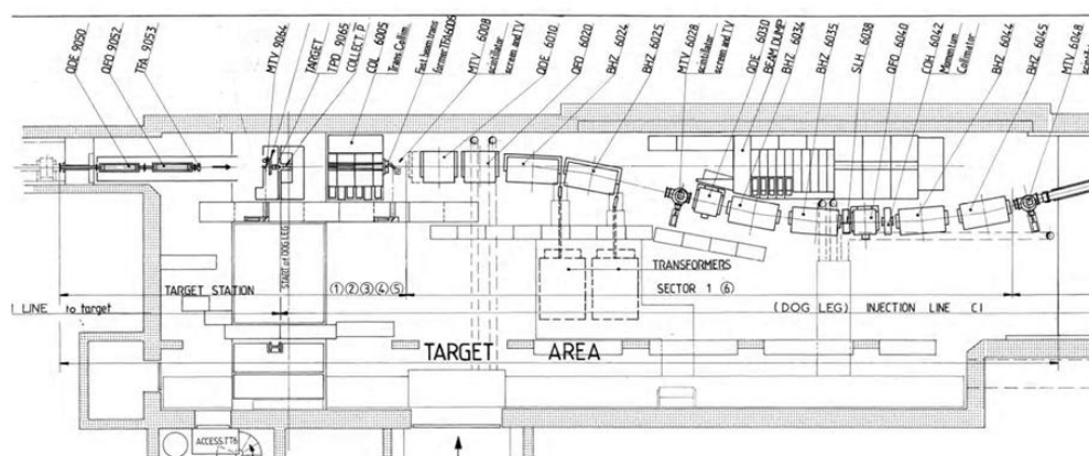
Fig. 1: The AD-target area technical drawing with the antiproton beam production and bending/focusing elements [7].
