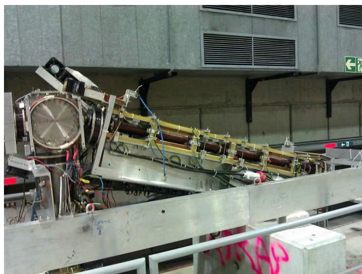
Solenoid positron transport coil for the ATRAP experiment. (spare module)
