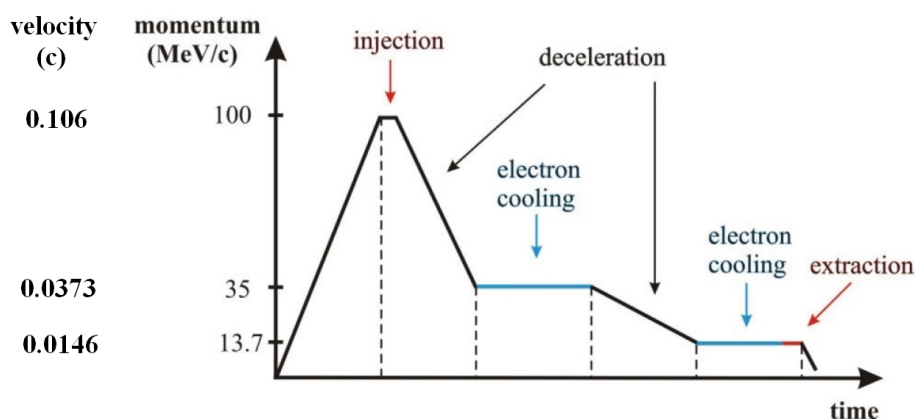
Fig. 7: A schematic view of the ELENA cycle
